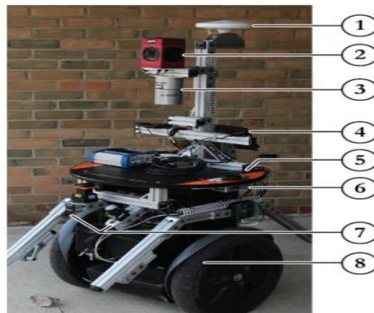
Figure 2: Segway robotic platform with Sensors outfit (Source: Carlevaris-Bianco, Ushani & Eustice ,2016).
